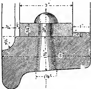
Fig. 5344. RIVET FASTENING.
